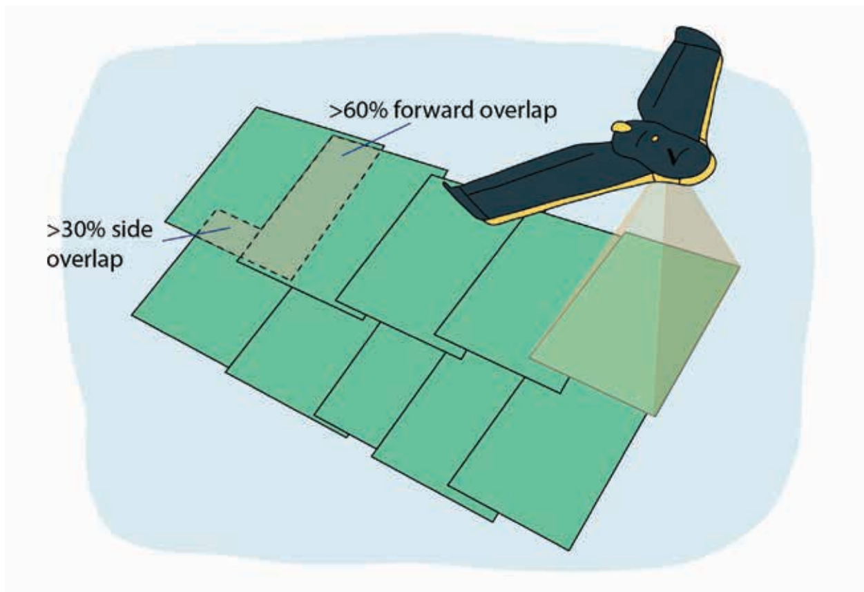
FIGURE 8. Recommended forward and side overlaps to create a mosaic with good positional accuracy.
